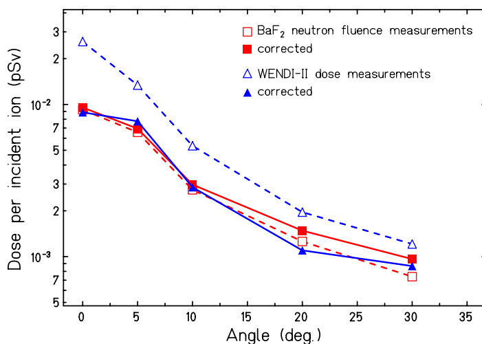
Figure 13. Neutron dose angular distributions for 200 MeV \text{u}^{-1} ^{12}\text{C} ions stopping in a 12.8 cm thick water target. Neutron doses at 3 m distance from the target were obtained by convolution of neutron fluences measured with a \text{BaF}_2 detector with the ambient dose equivalent h^*(10) . For comparison direct neutron dose measurements [32] using a WENDI-II detector are shown.
