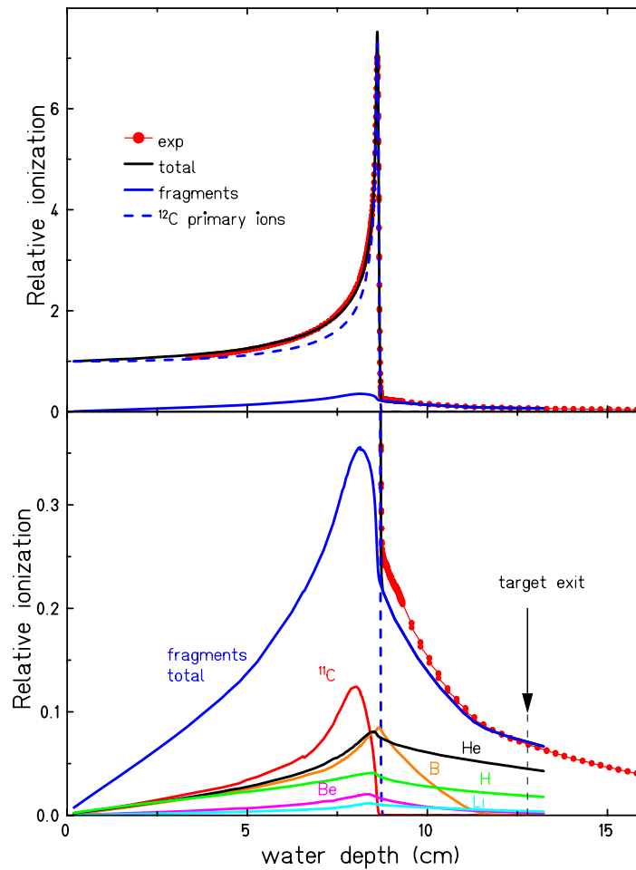
Figure 2. The ionization function (Bragg curve) of a 200 \text{ MeV u}^{-1} {}^{12}\text{C} ion beam in water. The measurement was performed with parallel-plate ionization chambers and a precision water absorber [5, 6]. Calculations with the Monte-Carlo code (particle and heavy ion transport code system (PHITS)) (see section 4) are in good agreement with the measurement. The lower part with magnified ordinate scale shows the contribution of fragments with different atomic numbers Z as calculated with PHITS. The thickness of the water target used in our fragmentation measurements is indicated by an arrow.
