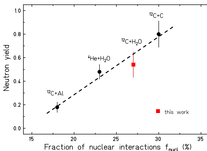
Figure 8. Measured neutron yields from [15]–[18] and this work versus the fraction f_{\text{nuc}} of ions undergoing nuclear interactions in the target (see table 1).
